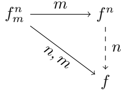
FIGURE 1. The diagonal limit. The solid arrows represent the limits or compactness properties available. The dashed arrow represents the limit we wish to establish.
